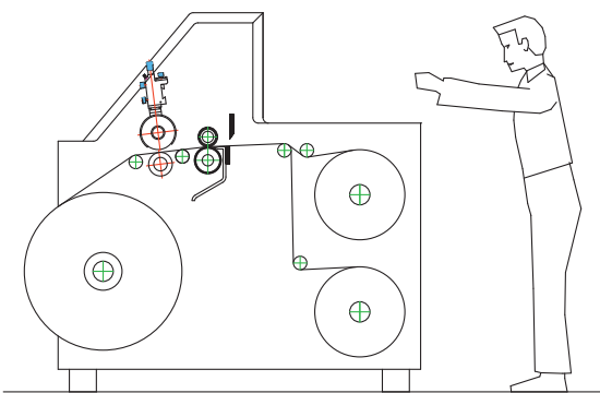
Slit-rewinding Mode
